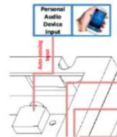
Input Jack for Mobile Phone Sound
