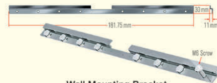
Wall Mounting Bracket
