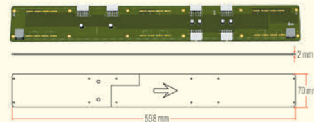
LED Interconnect Board
